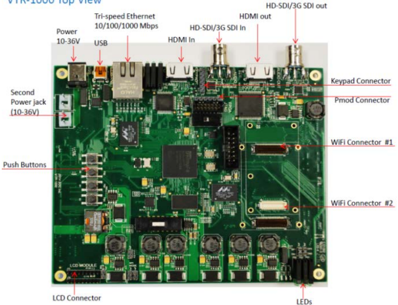
Fig.1 VTR-1000 Top View
