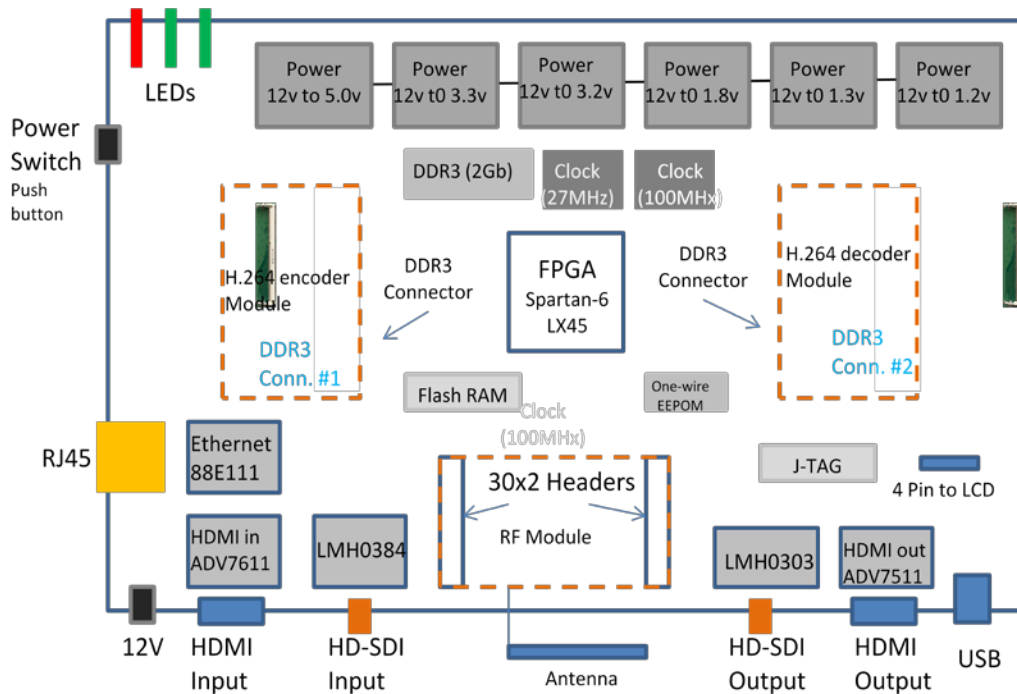
Fig.3 VTR-1000 Block Diagram
