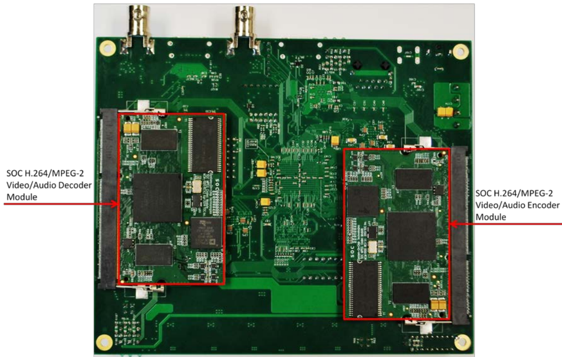
Fig. 2 VTR-1000 bottom View
